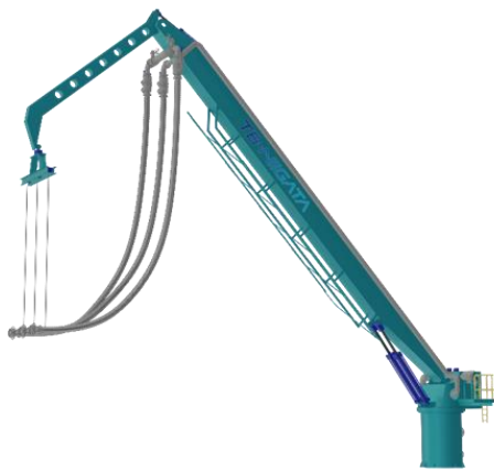
3D model of bunkering boom for ammonia
